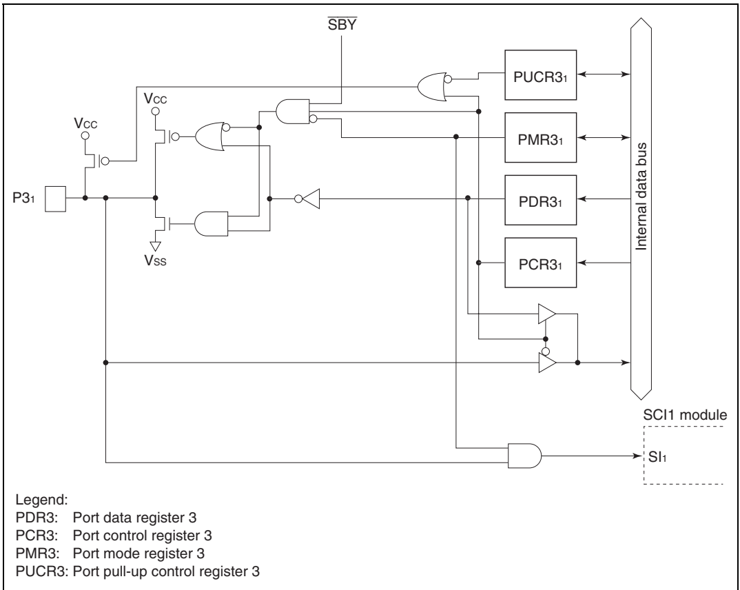
Figure C.3 (c) Port 3 Block Diagram (Pin P3 1 ; Function of H8/3857 Group Only)
