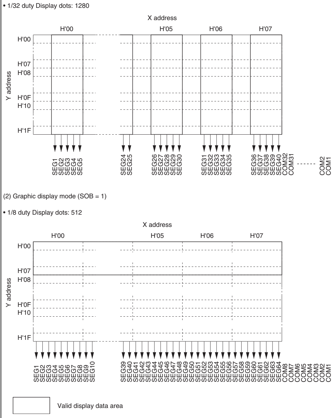
Figure 13.5 Display Duty and Valid Display Data Area (2)
