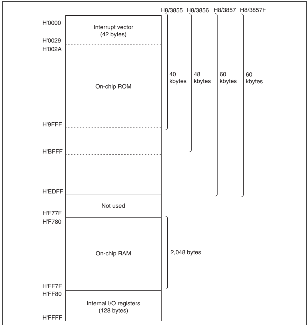
Figure 2.16 (a) H8/3857 Group Memory Map
