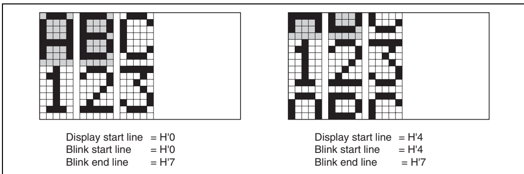
Figure 13.11 Blinking during Display Scrolling (SOB = 0, 1/16 Duty)
