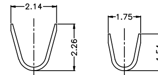
A-A SECTION B-B SECTION
