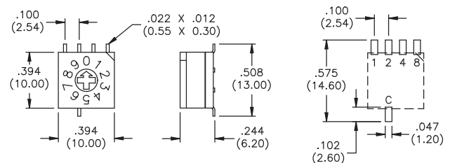
Mechanical outline
