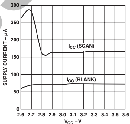
TPC 8. Supply Current vs. Voltage
