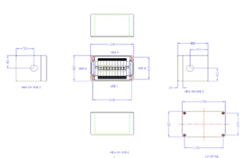
JB-FT10 Drawing
