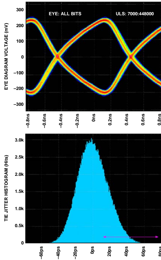
Figure 60. Data Eye for LVDS Outputs in ANSI-644 Mode with Trace Lengths Greater Than 24 Inches on Standard FR-4, External 100 Ω Far Termination Only
