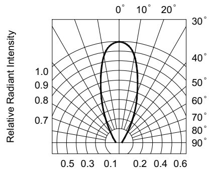
FIG.6 RADIATION DIAGRAM
