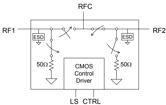
Figure 1. Functional Diagram
