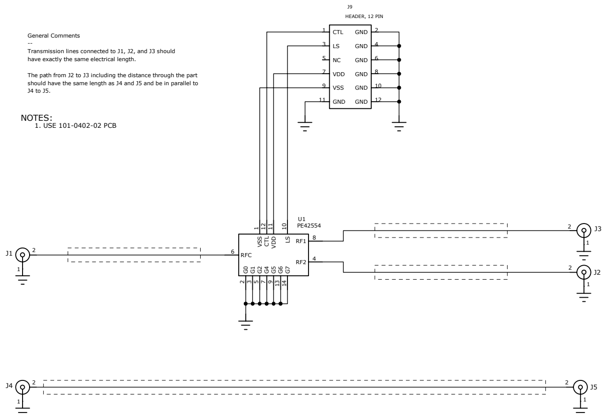
Figure 7. Evaluation Board Schematic Peregrine Specification 102/0478
