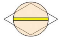
INCORRECT orientation of Gotcha Stick (penetrates barrier guard opening even though human shape DOES NOT)
