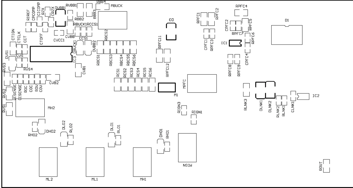
Bottom Assembly
