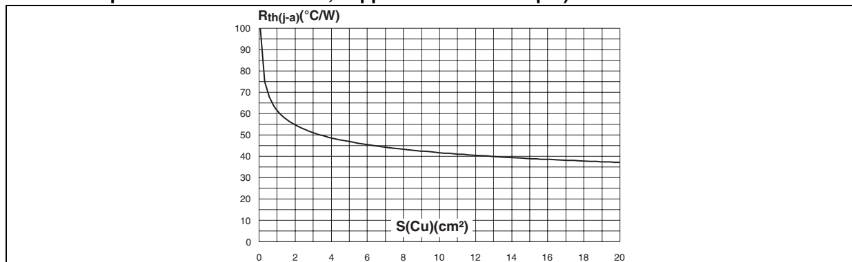
Figure 11. Thermal resistance junction to ambient versus copper surface under tab (Epoxy printed circuit board FR4, copper thickness = 35 µm) for DPAK
