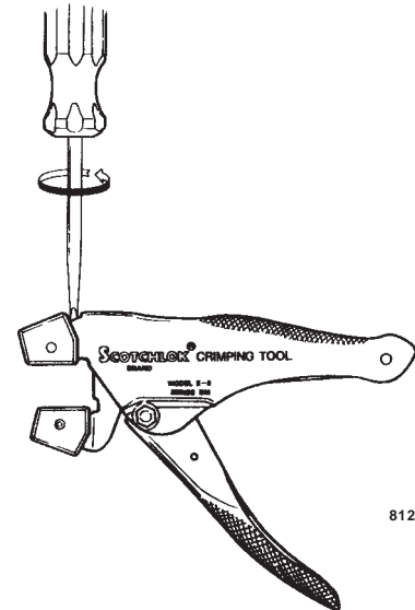
Figure 1. Removal of jaw inserts
